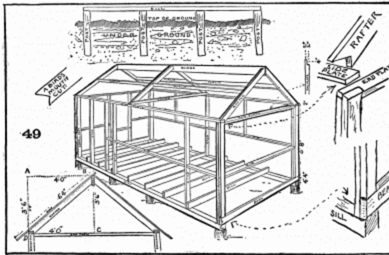
Frame of two-by-fours milled lumber, with names of parts.
