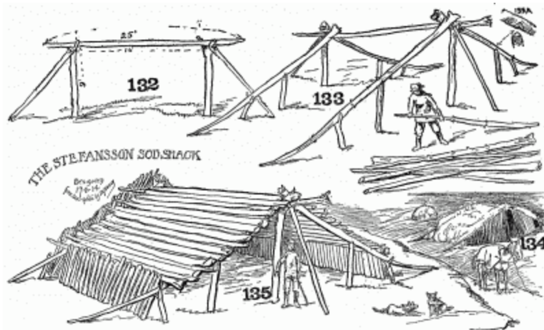
Details of the Stefansson sod shack.
