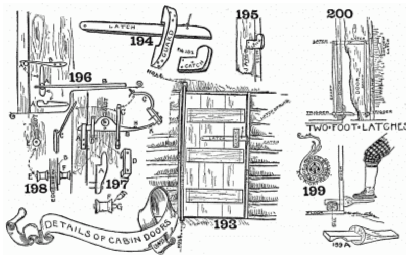
Foot and thumb door-latches.
