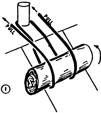
Parbuckling
