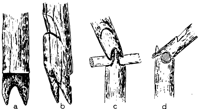
RAFTER END LOWER RAFTER END, AT POST AND WALL PLATE POST, WALL PLATE, RAFTER AT POST AND WALL PLATE
