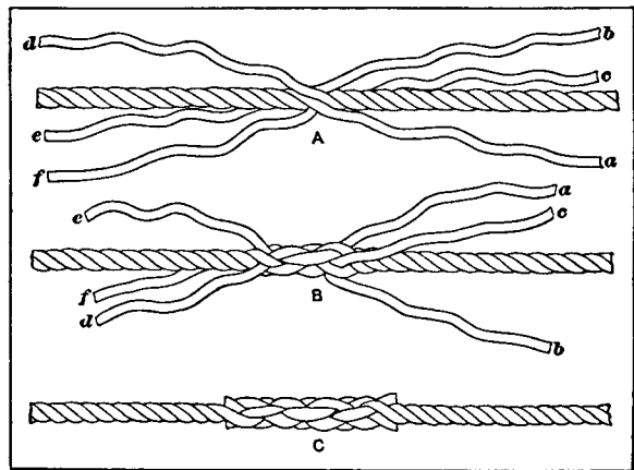
Fig. 1. Method of Making a Short Splice
