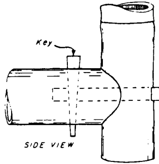
TENON KEY JOINT FOR HEAVY DUTY OR FINE WORK
