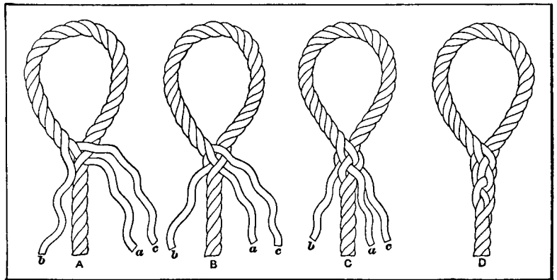
Fig. 3. Method of Making an Eye-splice
