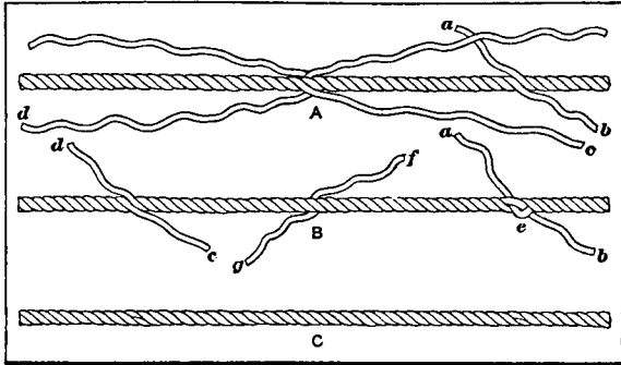
Fig. 2. Views illustrating how a Long Splice is made
