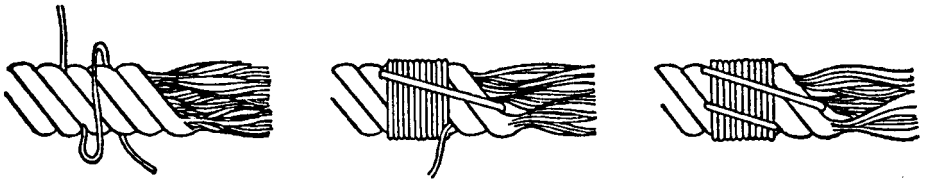
(l) palm and needle whipping
