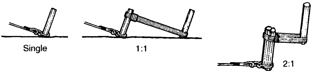
Figure A18.1 Combinations of picket holdfasts
