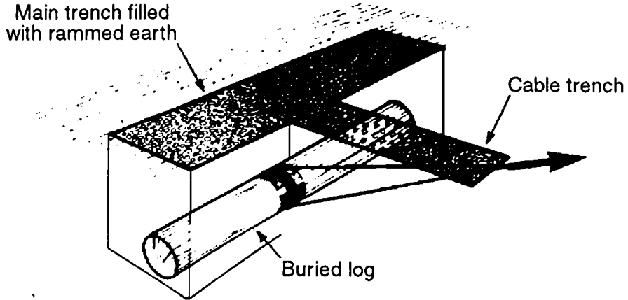
Figure A18.3 A buried log anchorage
