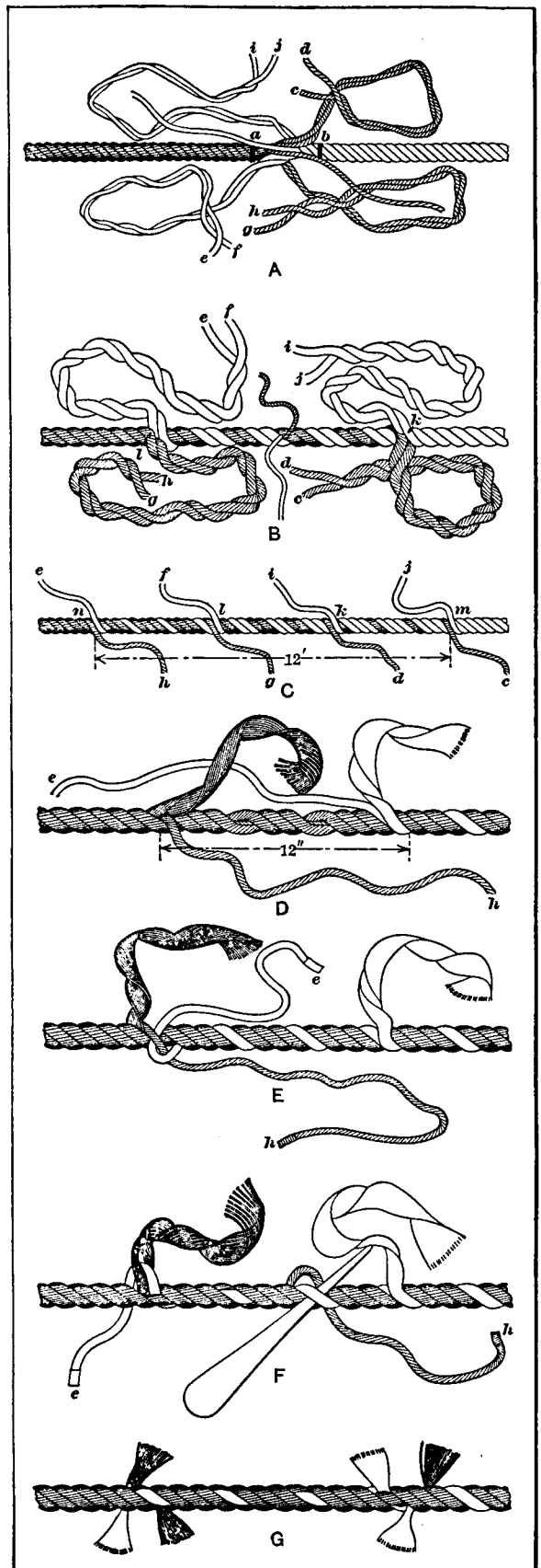
Fig. 4. Splicing Manila Transmission Rope
