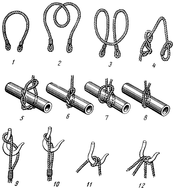
Fig. 230. Hoisting slings and knots
