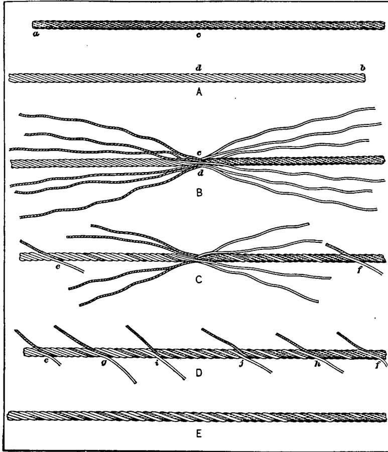
Fig. 5. Method of Splicing a Six-strand Wire Rope
