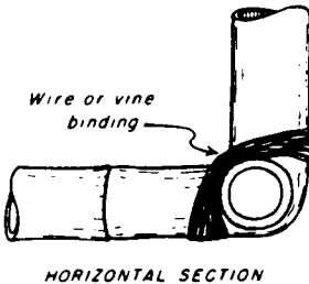
DOUBLE BUTT BENT JOINT Suitable for furniture and similar uses
