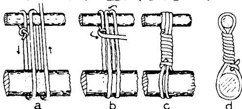
LASHING RIDGEPOLES TOGETHER
