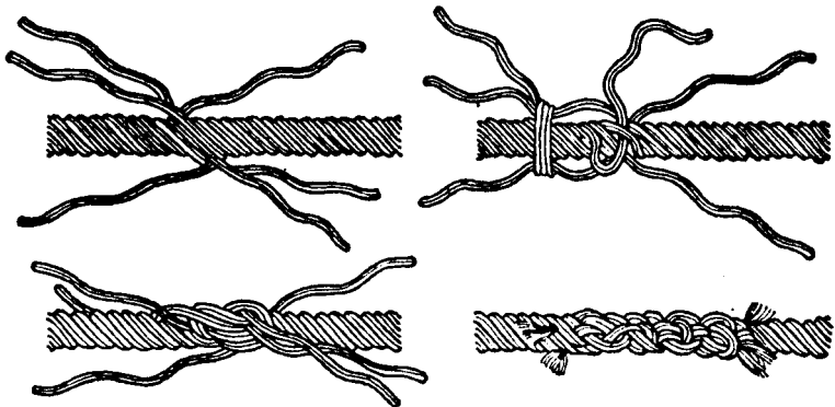
(k) short splice
