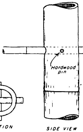
JOINT FOR CONNECTION OF SMALL MEMBERS TO LARGE MEMBERS
