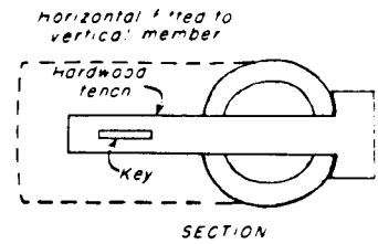
TENON KEY JOINT FOR HEAVY DUTY OR FINE WORK
