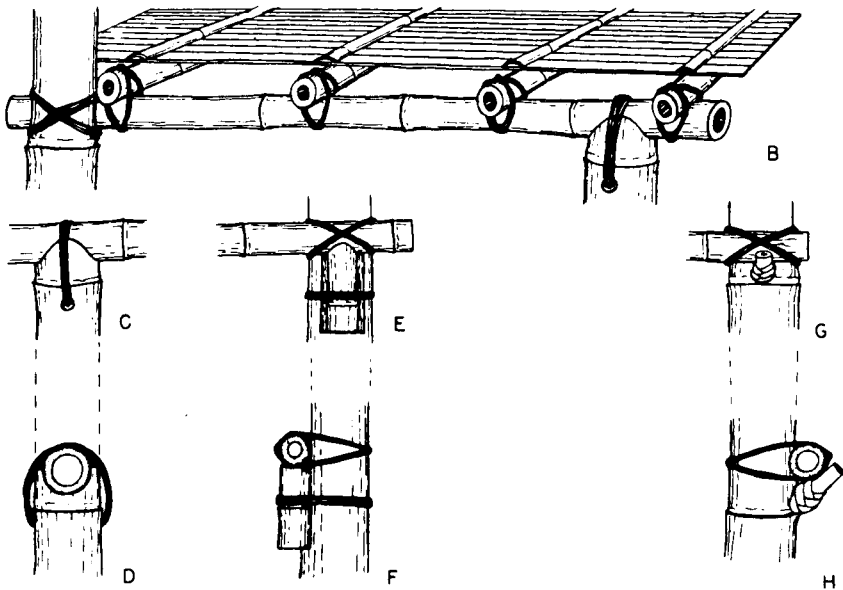
Figure 10 --Details of bamboo construction: A , fitting and binding culms at joints in roof and frame; B , fitting and securing bamboo boards of floor; C and D , saddle joint; E and F , use of inset block to support horizontal load-bearing elements; G and H , use of stump of branch at node of post to support horizontal load-bearing elements.
