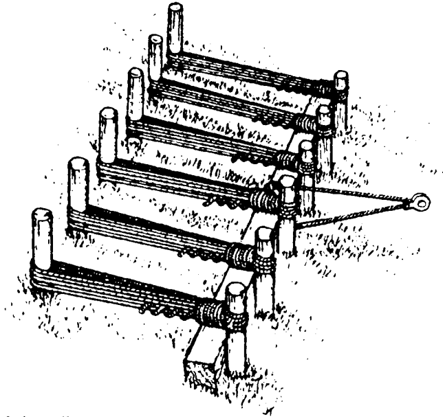
Figure A18.2 A baulk anchorage
