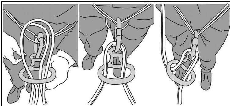
Figure 9-27. Figure-eight descender
